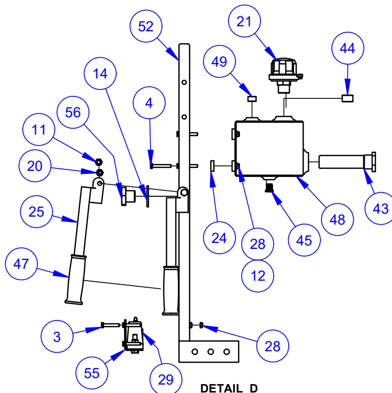
DETAIL D
