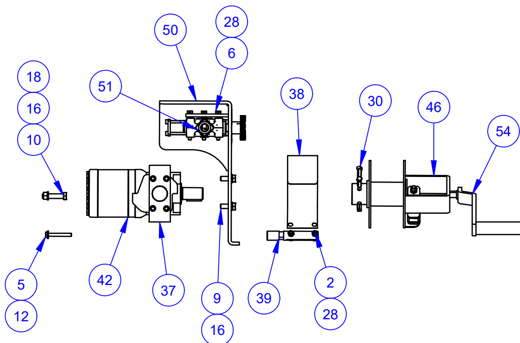
DETAIL C
