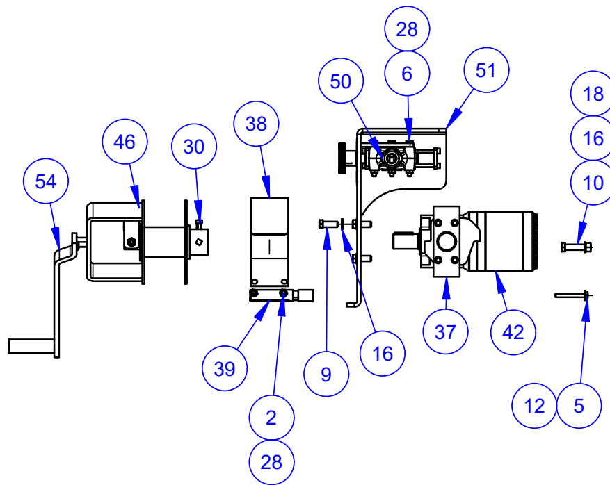
DETAIL C
