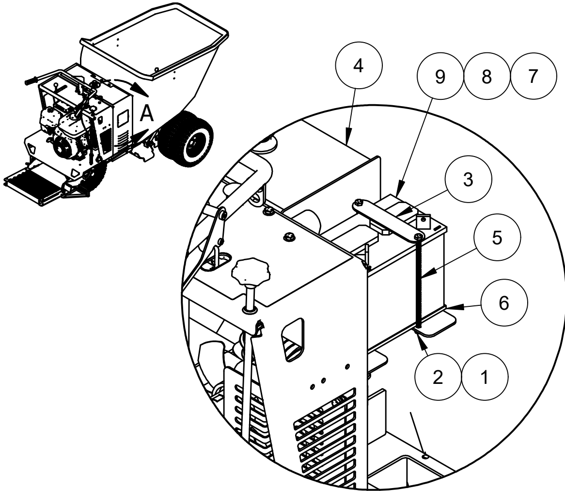
DETAIL A PARTS HIDDEN FOR CLARITY
