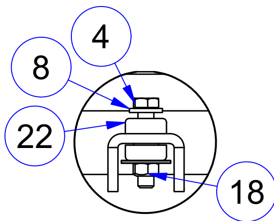
DETAIL: POWER UNIT MOUNT
