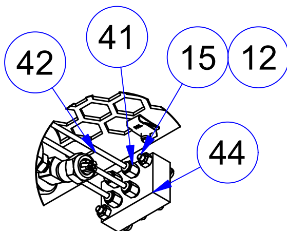
DETAIL: GREASE BLOCK
