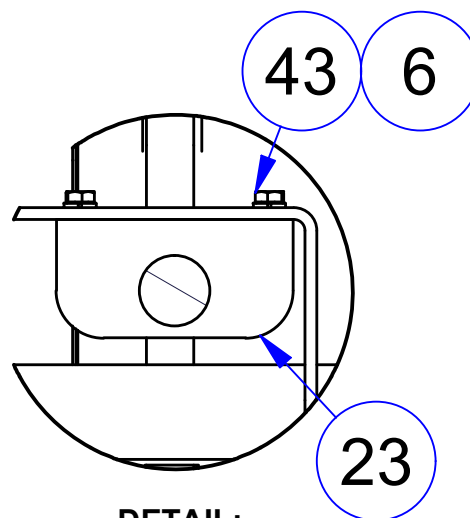
DETAIL: BEARING BLOCK
