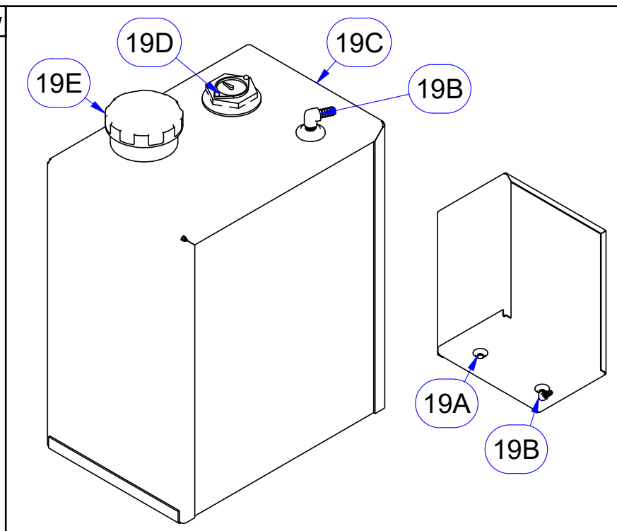
075643 Tank Assembly
