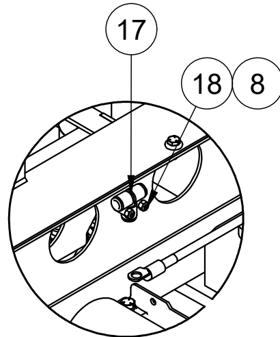
DETAIL SPRAY TEE FITTING
