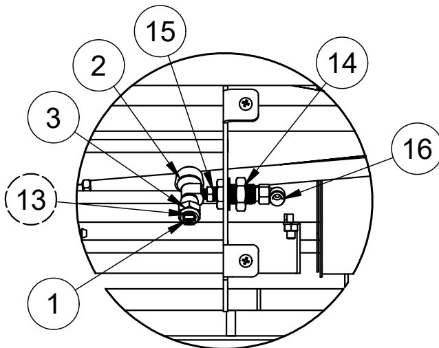
DETAIL SPRAY NOZZLE
